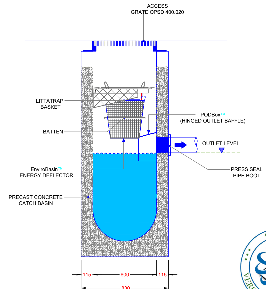
SECTION B-B
