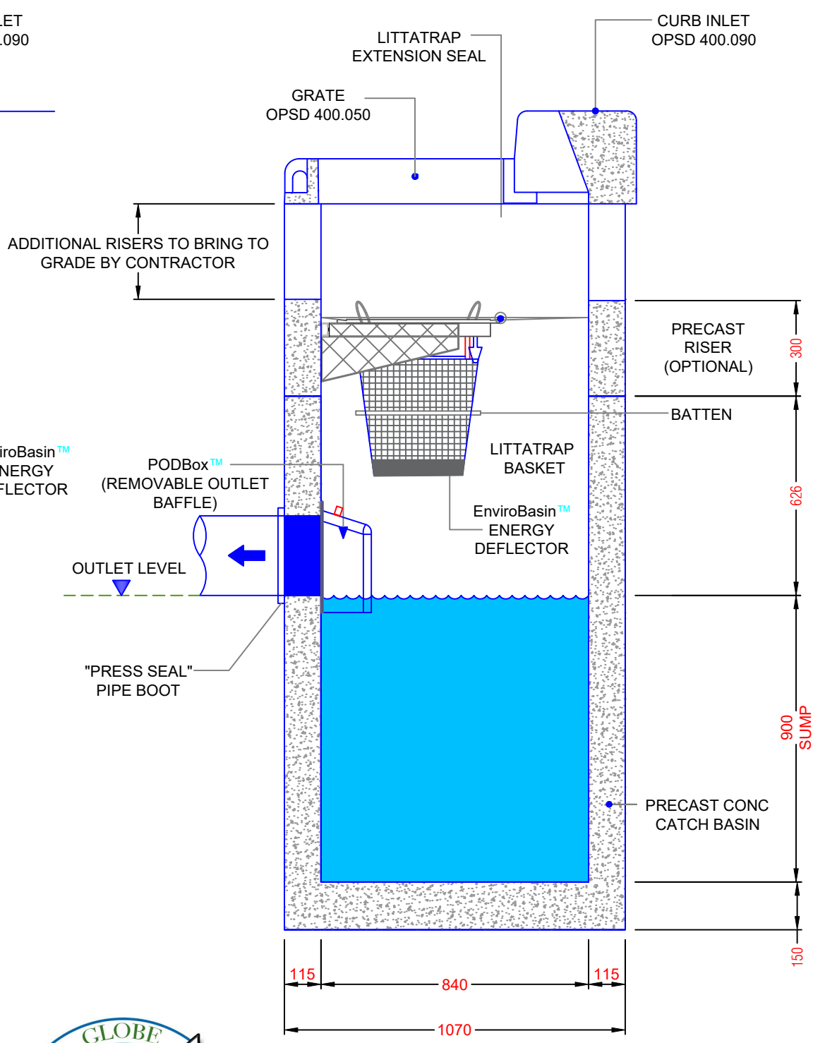
SECTION B-B
