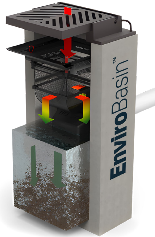
EnviroBasin™ Standard Grate Inlet
