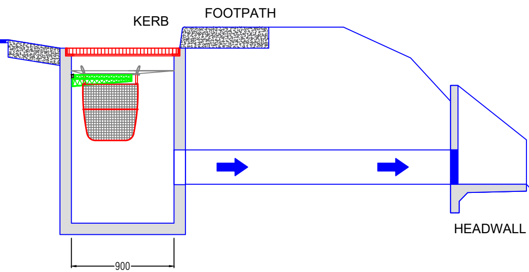
ENVIROPOD200 (900x900mm GULLEY PIT)
